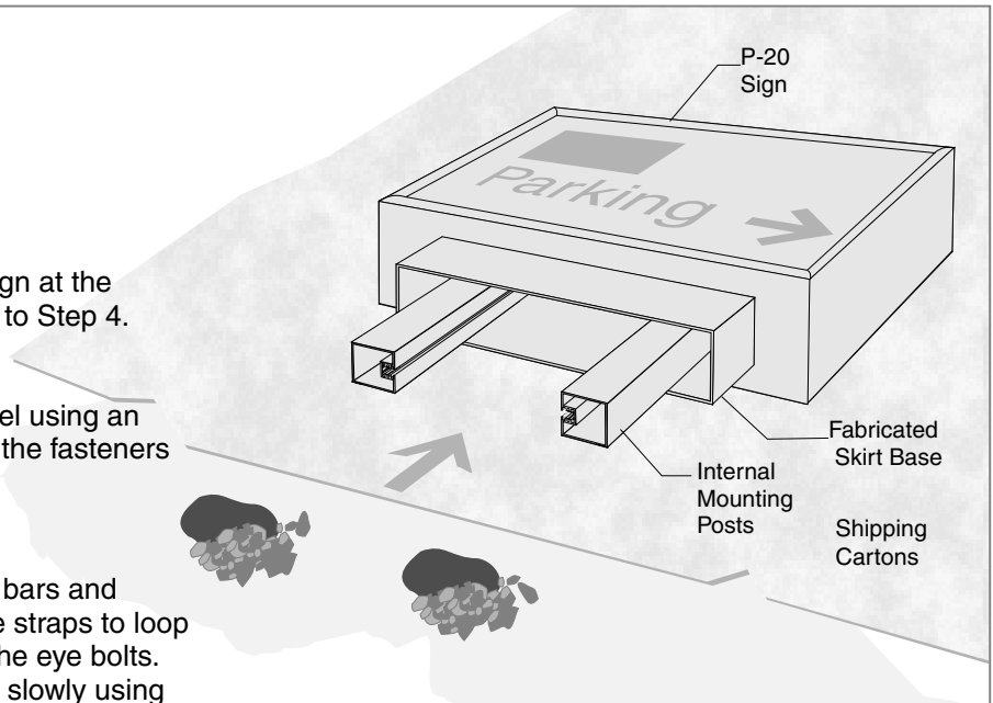
Pylons with Internal Posts
