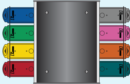
STANDARD TABS FINGOOD: HIDPF-R8511-8 MINIMUM WALL CLEARANCE: 19"
